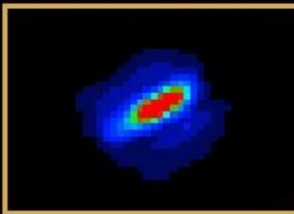
Mid-Infrared : IRAS
