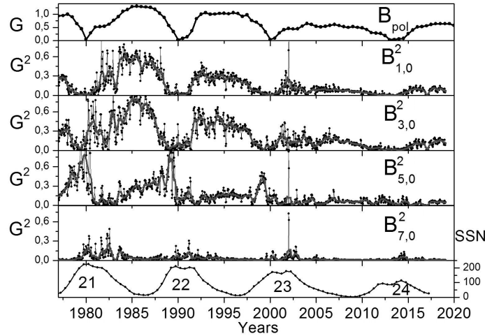
Figure 1: Time dependence of the squared magnetic field connected with the first odd axisymmetric harmonics up to l = 7 [1]. The lowest plot represents the time variation of sunspot numbers (SSN) with the cycle numbers indicated; the top plot is the polar field.
